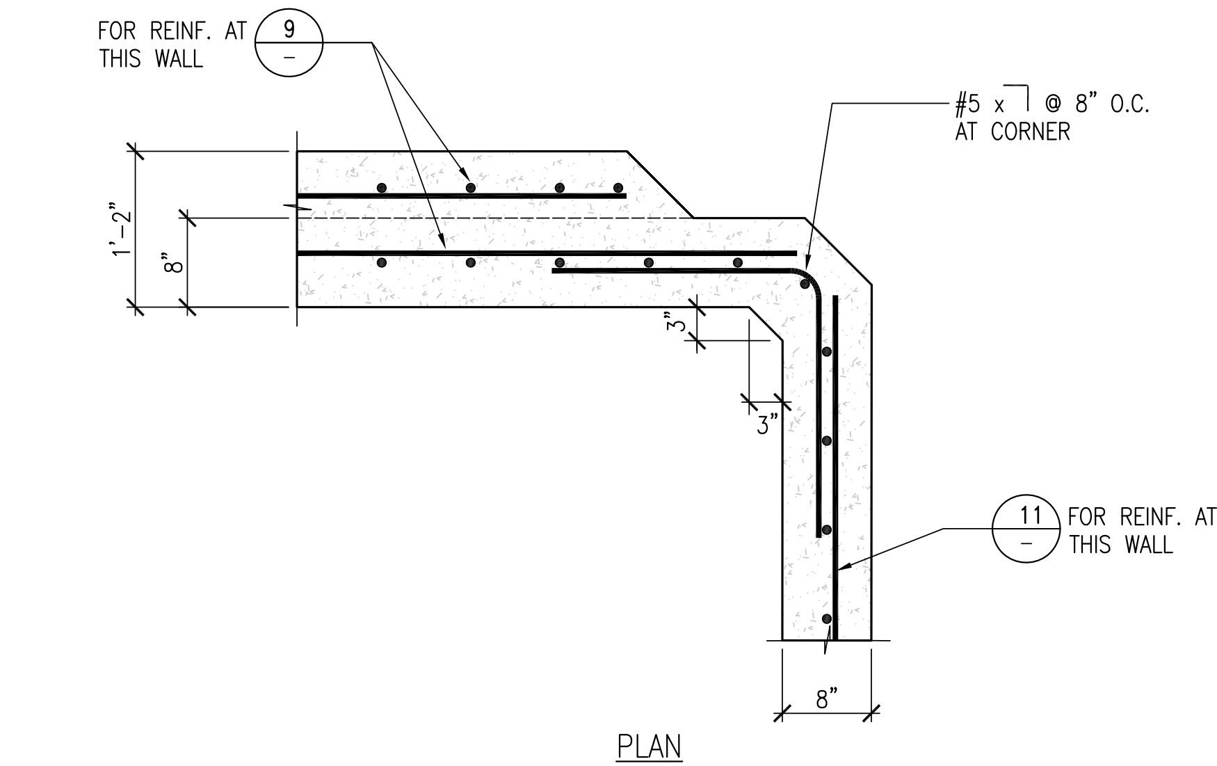
STATUE PEDESTAL WALL CORNER REINFORCING
