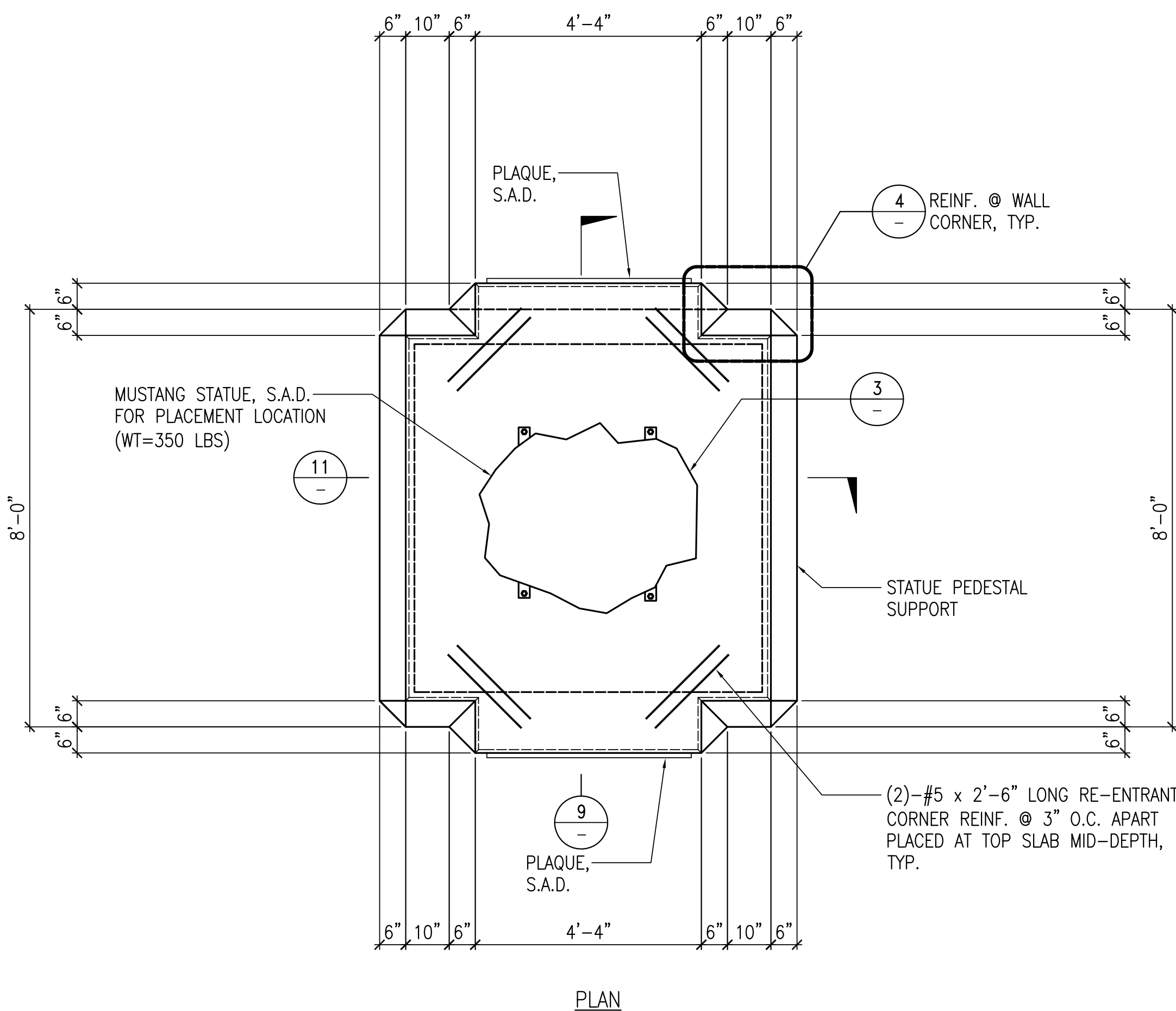
STATUE BASE ANCHORAGE
