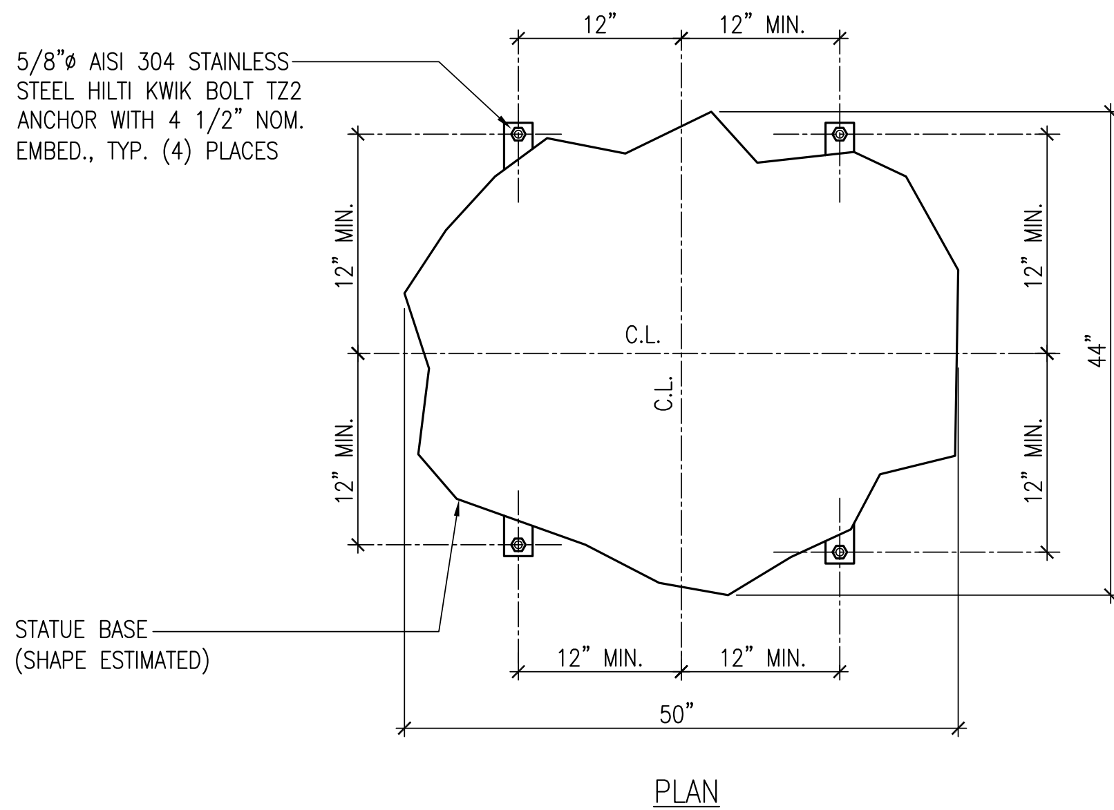
STATUE BASE ANCHORAGE
